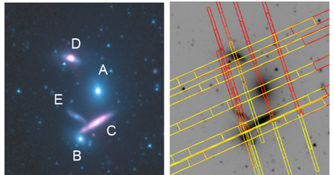
Figure 2. IRS sampling (Long-Low; \sim 10'' \times 5'' and Short-Low; \sim 3'' \times 6'' slits) shown on HCG 40 (IRAC four-color image of \sim 4' \times 4' shown on the left, IRAC 3.6\mu\text{m} image shown on the right). First-order spectral coverage is shown in yellow with second order in red. It should be noted the mapping combined with staring strategy probes the intragroup region, as well as the galaxies themselves.
