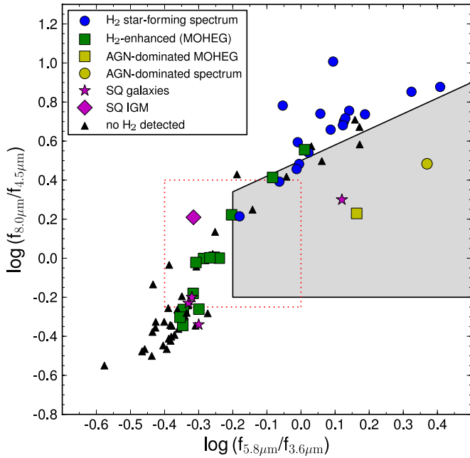
Figure 10. IRAC color-color diagram for the sample; H 2 -enhanced galaxies (MOHEGs) are shown as green squares, H 2 -detected galaxies are shown as blue circles. The red dashed box shows the underpopulated region in color-color space from Walker et al. (2010). The shaded area corresponds to the AGN color selection criteria of Lacy et al. (2004); AGN-dominated systems (as determined by their mid-infrared spectra) are in yellow. The purple diamond is the location of the shocked IGM in SQ (from Cluver et al. 2010), with SQ member galaxies shown as magenta stars.
