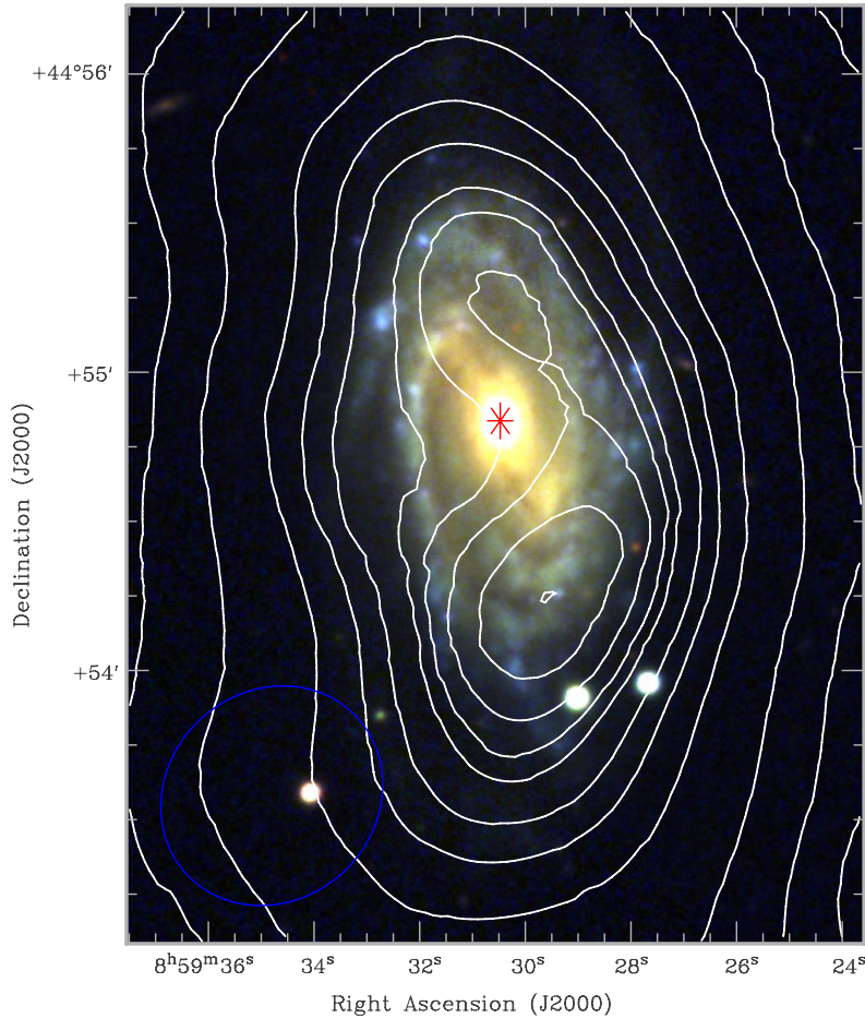
Figure 3. Optical SDSS u g r composite of CIG 292 with overlaid H I contours. The contours are presented as white solid lines and correspond to levels of 1.2, 3.7, 6.2, 7.6, 8.5, 9.5, 10.0, 10.6, 11.4, and 12.1 \times 10^{20} at \text{cm}^{-2} . The optical center of the galaxy is indicated with a red star and the beam is shown in the bottom left of the image. (A color version of this figure is available in the online journal.)
