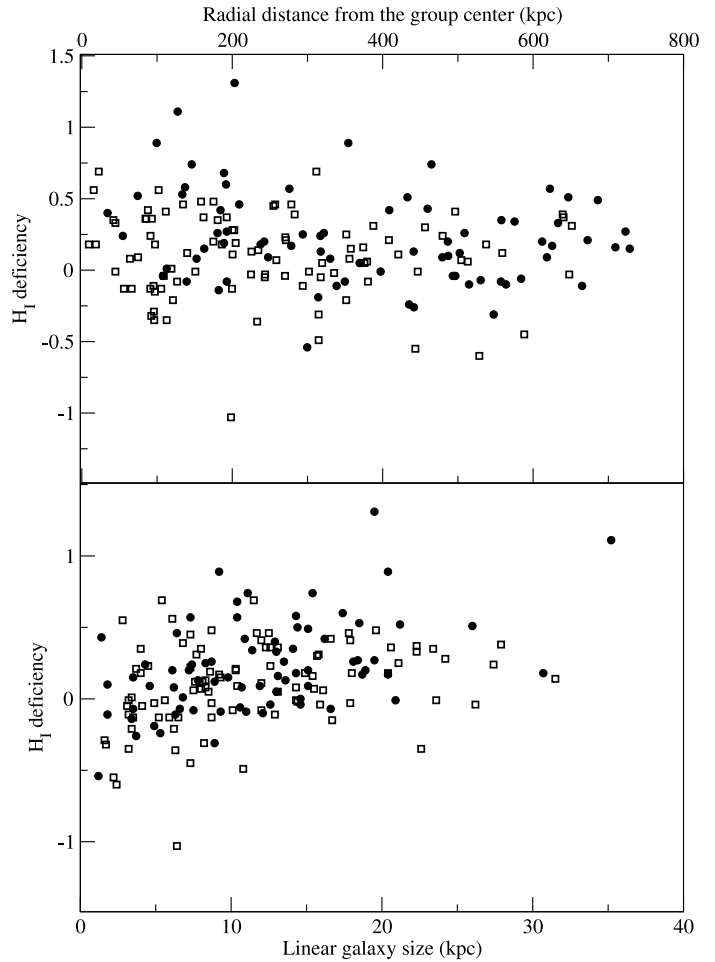
Figure 1. The top panel shows the distribution of H I deficiency with respect to the distance from the group centre. The bottom panel shows the distribution of H I deficiency with respect to the linear sizes of the galaxies. The number of galaxies in groups with and without Xray emission are 74 and 96, respectively.
