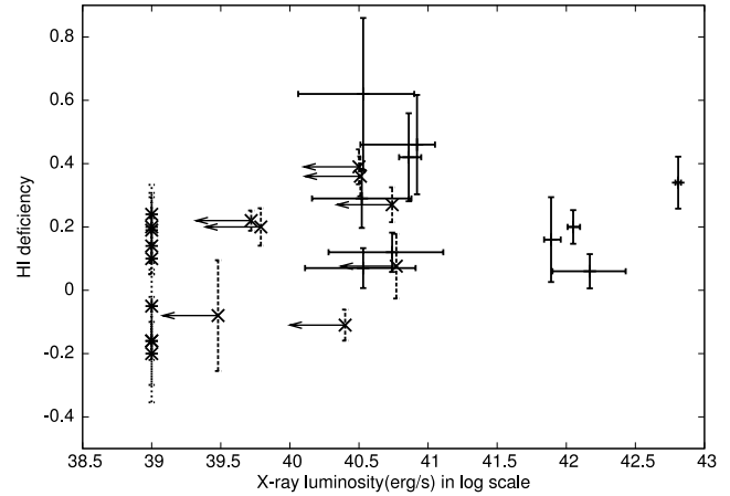
Figure 3. Variation in H I deficiency with L_x is shown.
