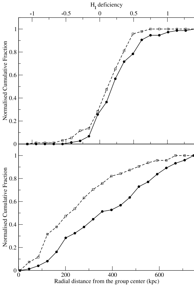
Figure 2. The top panel shows the behaviour of normalised cumulative fraction of the two sets of galaxies with respect to the H I deficiency; the bottom panel shows the same with respect to the radial distances from their group centres. Filled circles connected by solid lines represent galaxies in X-ray bright groups whereas empty squares connected by dashed lines represent galaxies in non X-ray groups
